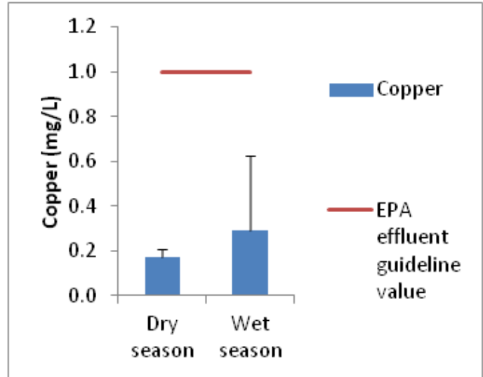
Figure 17. Cu in wastewater
