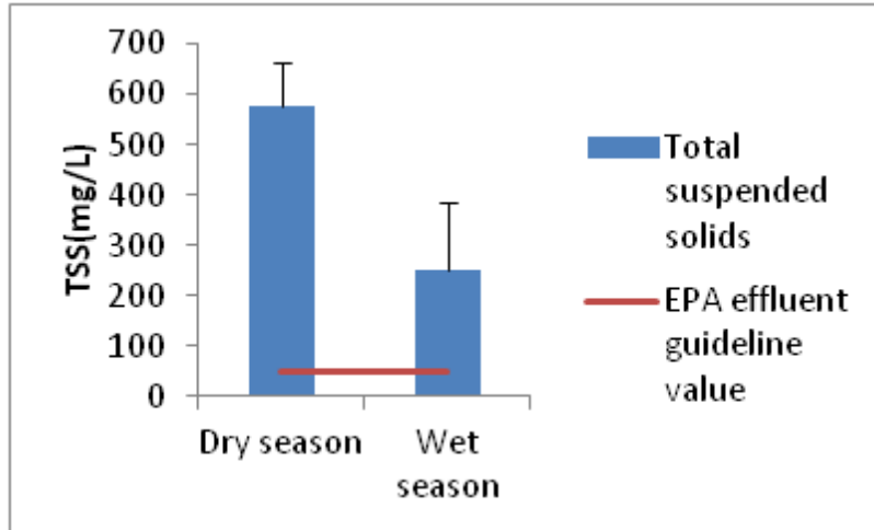
Figure 8. Total suspended solids in wastewater
